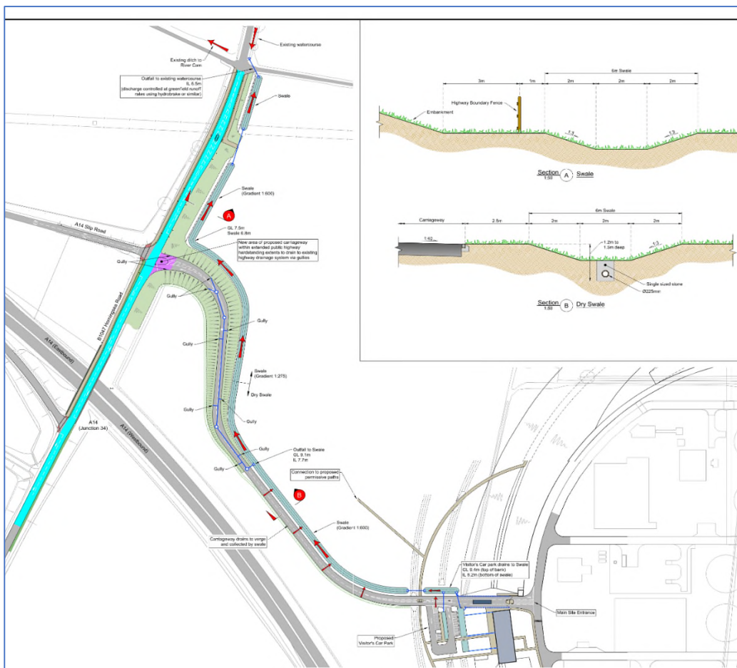
Figure 5.1: Proposed Access Road Surface Water Drainage
